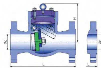
CLASS 1500 - 2500
