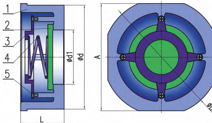
EXECUTION PN
