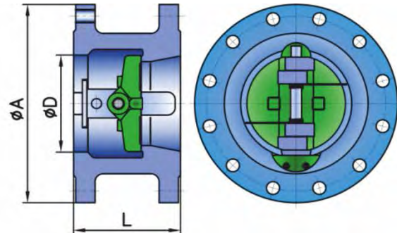
FLANGE MOUNTED TYPE
