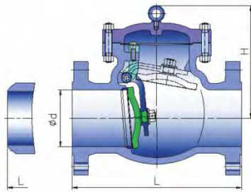
CLASS 150 - 300
