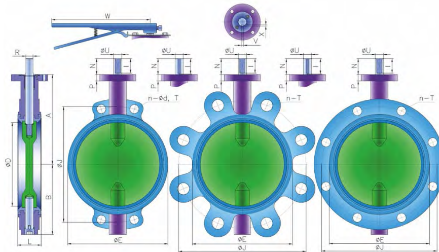
WAFER TYPE
